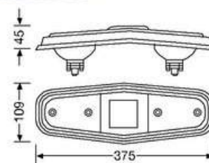
Minibus Tail Lamp
