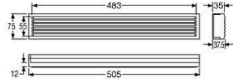
Order No: 2402DM Damper Şase Takoza Chock Support For Chassis
