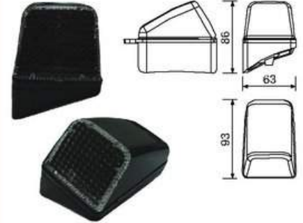
FH12 VV Cabin Top-Ceiling Corner Lamp
