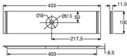
Order No: 2446DM Damper Şase Takoza Chock Support For Chassis
