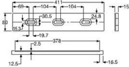
Order No: 2401DM Damper Şase Takoza Chock Support For Chassis
